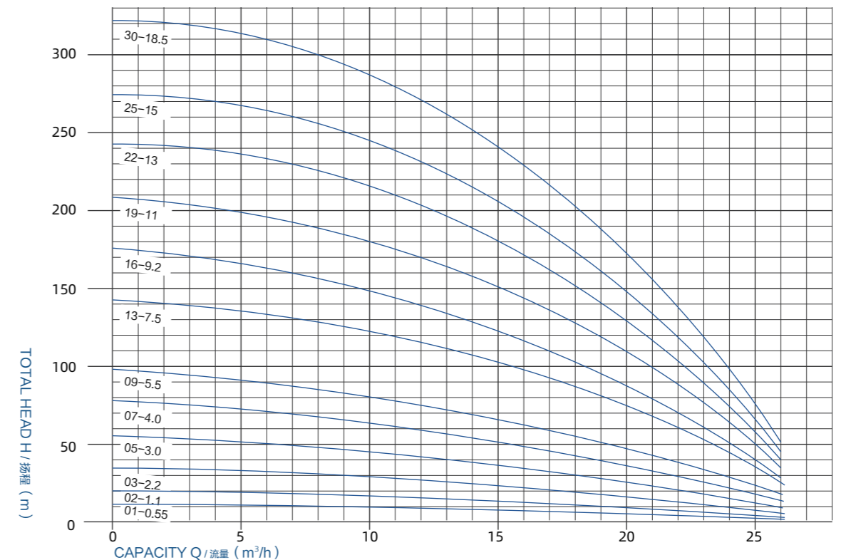
5SP15 SUBMERSIBLE PUMPS
