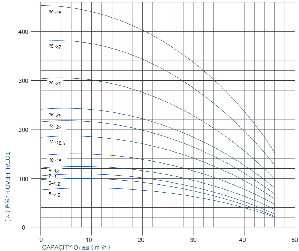
6SP32 SUBMERSIBLE PUMPS
