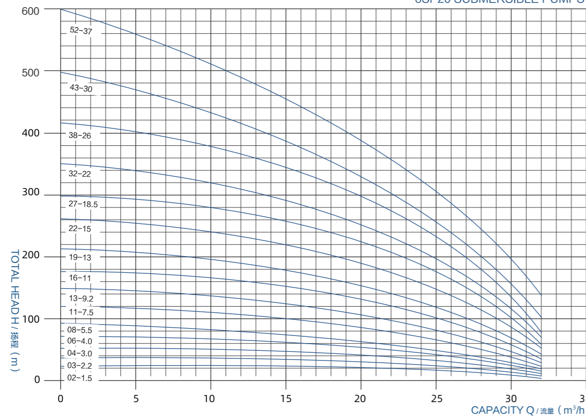
6SP20 SUBMERSIBLE PUMPS
