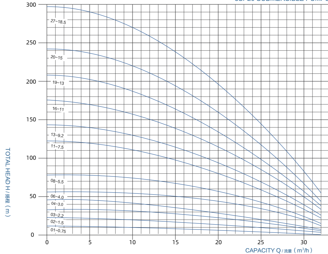
5SP20 SUBMERSIBLE PUMPS
