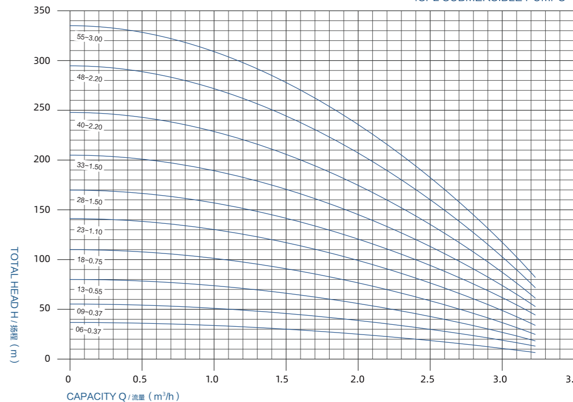
4SP2 SUBMERSIBLE PUMPS
