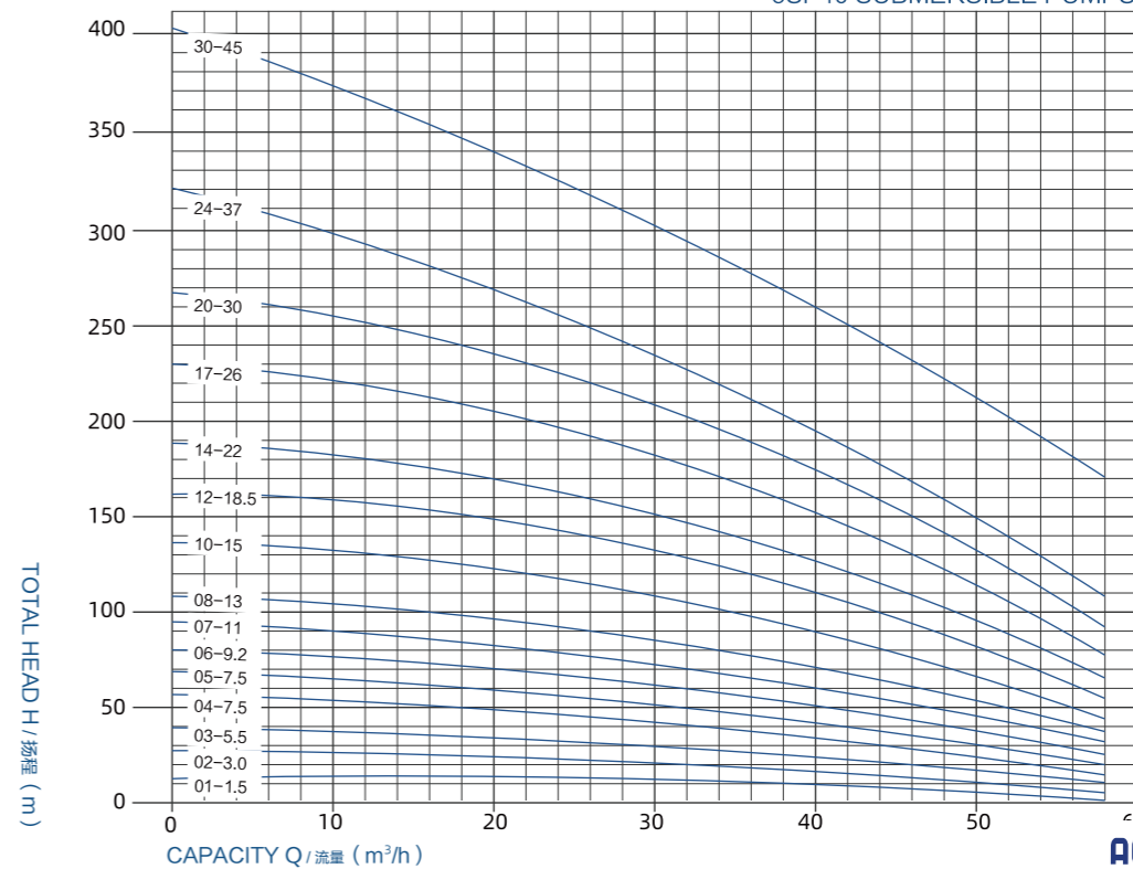
6SP40 SUBMERSIBLE PUMPS
