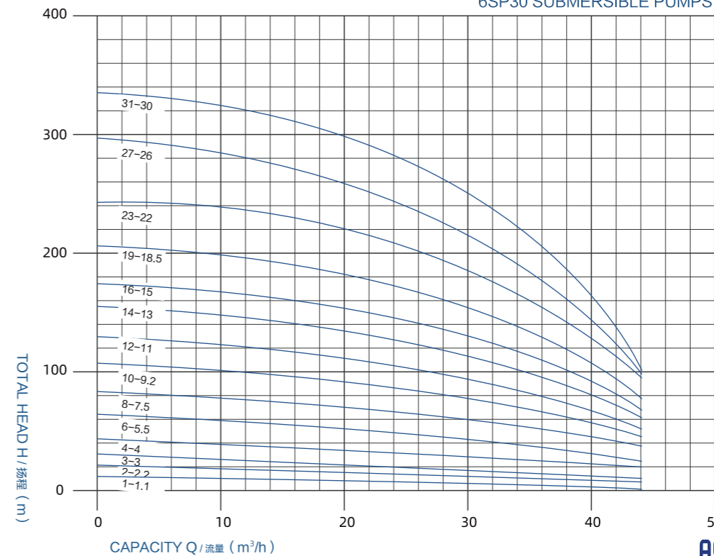
6SP30 SUBMERSIBLE PUMPS
