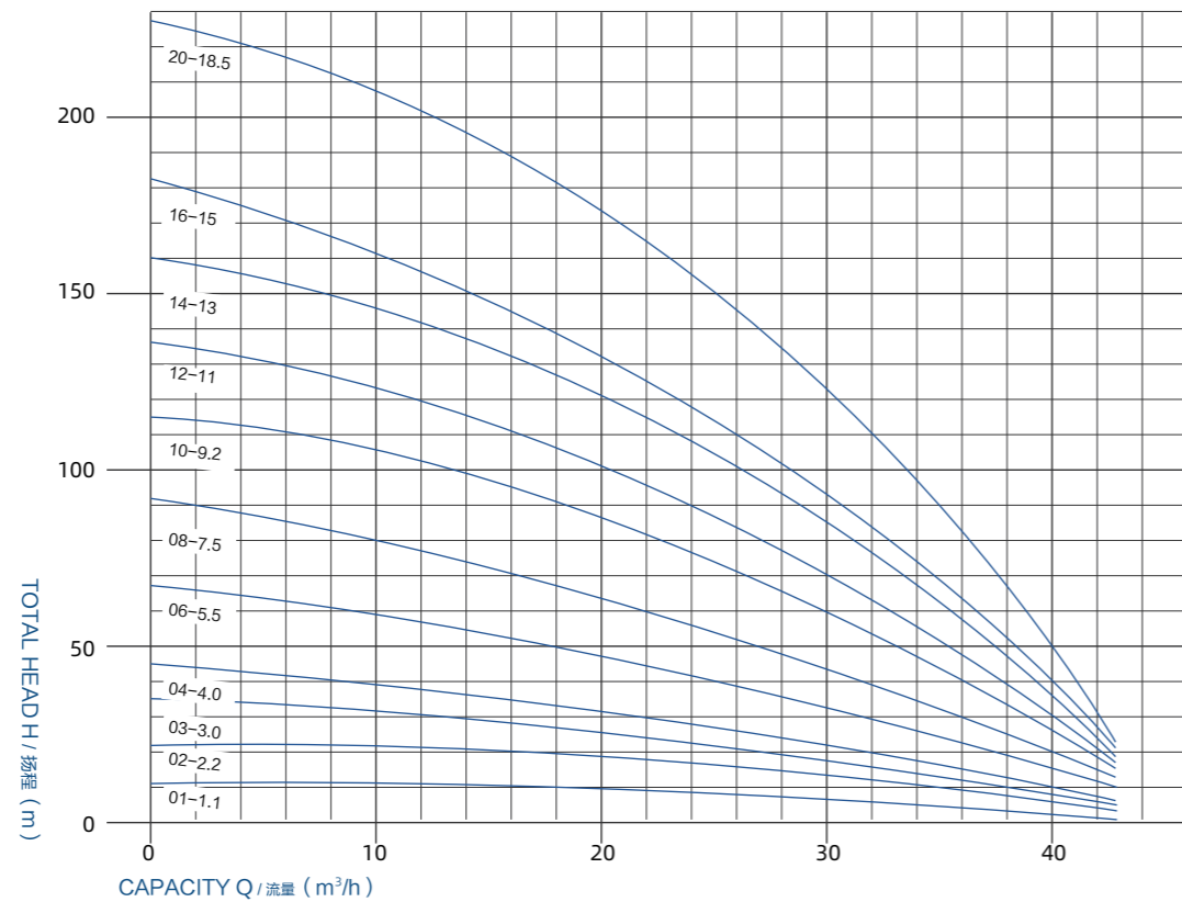
5SP30 SUBMERSIBLE PUMPS
