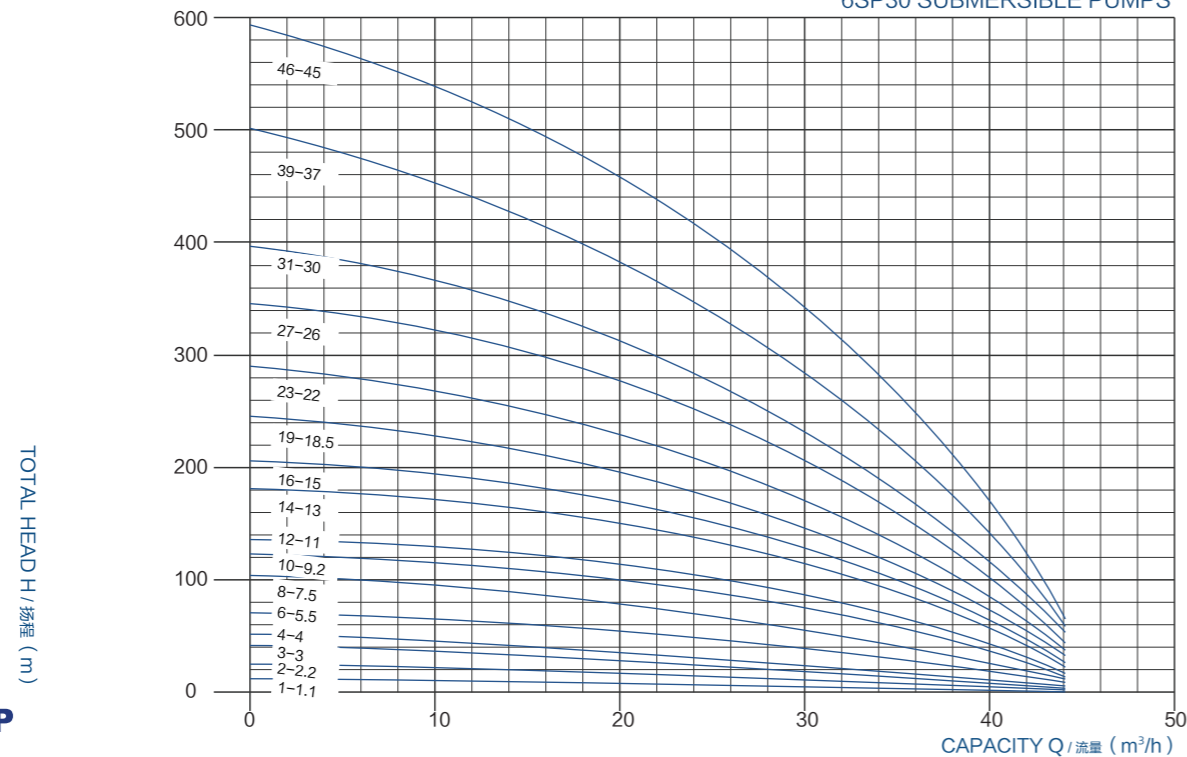
6SP30 SUBMERSIBLE PUMPS
