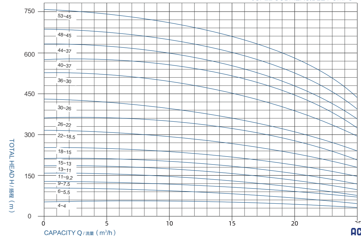
6SP22 SUBMERSIBLE PUMPS
