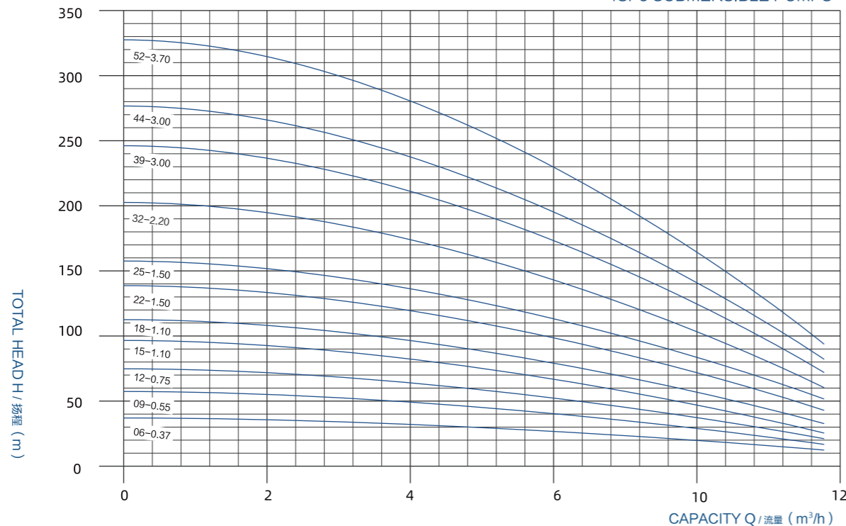
4SP3 SUBMERSIBLE PUMPS
