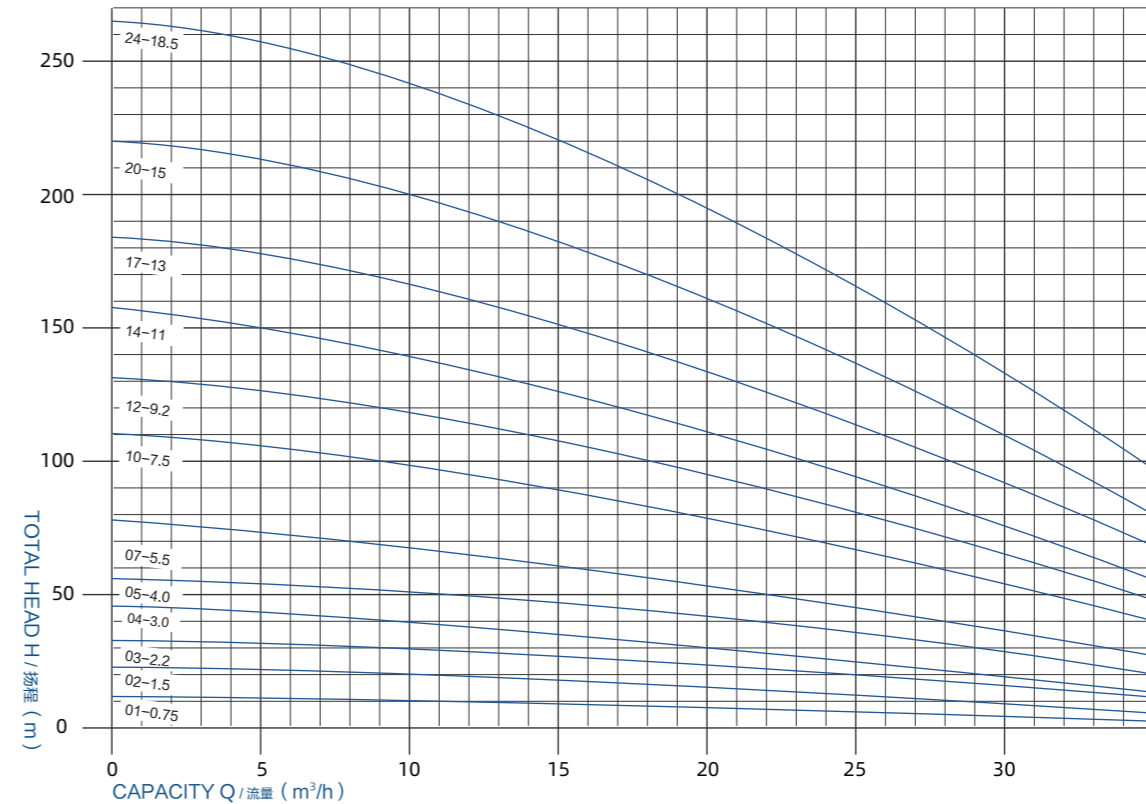
5SP25 SUBMERSIBLE PUMPS
