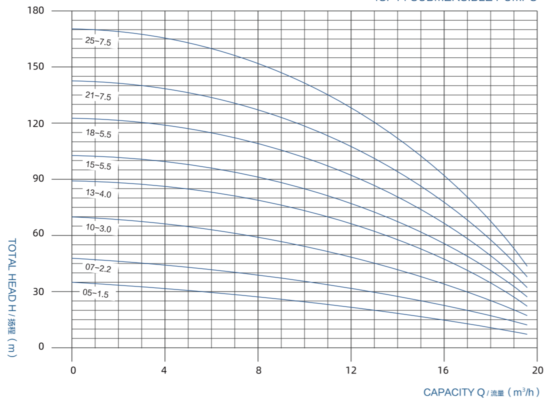
4SP14 SUBMERSIBLE PUMPS
