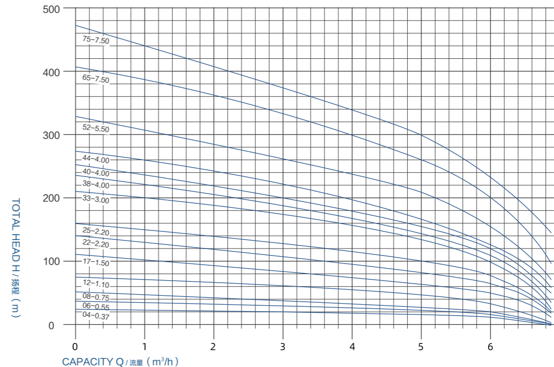
4SP5 SUBMERSIBLE PUMPS
