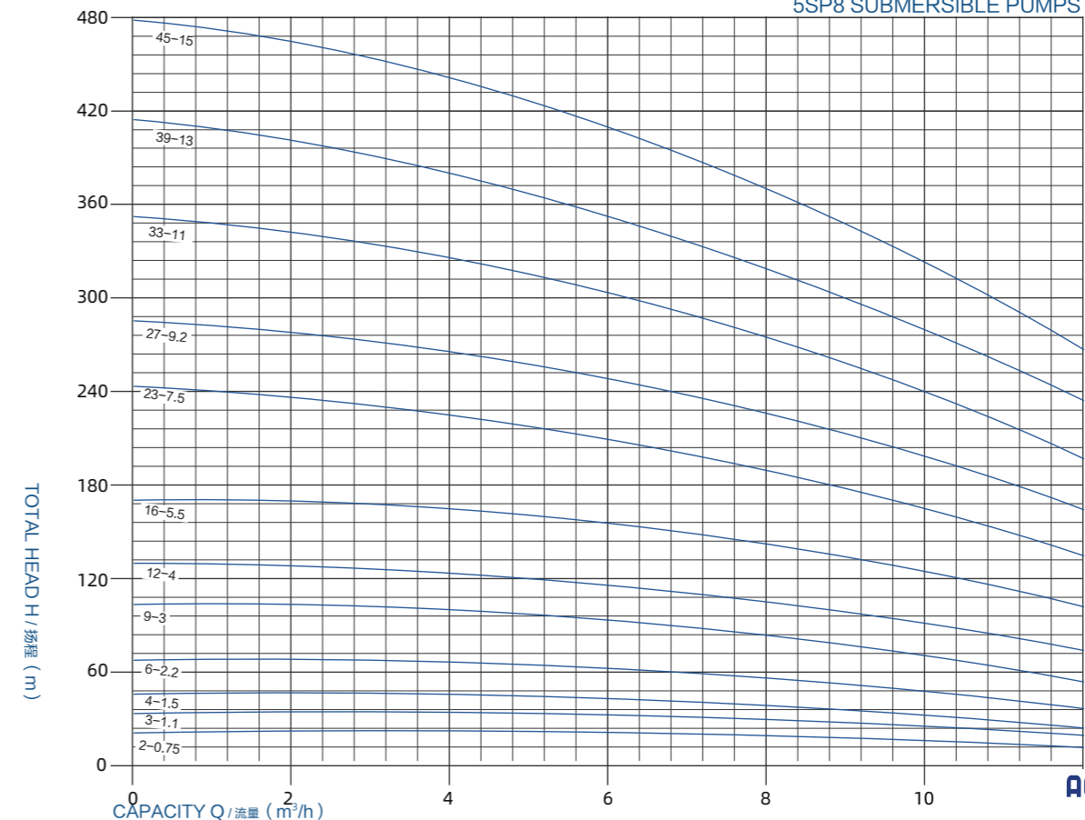
5SP8 SUBMERSIBLE PUMPS
