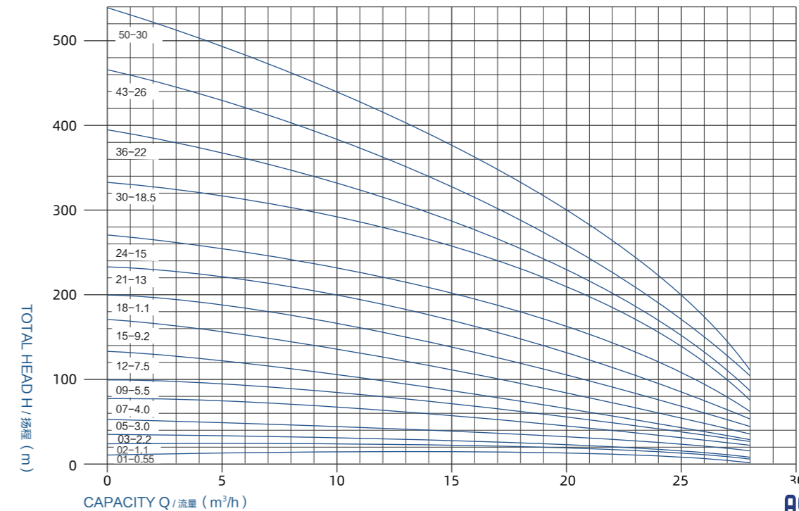
6SP17 SUBMERSIBLE PUMPS
