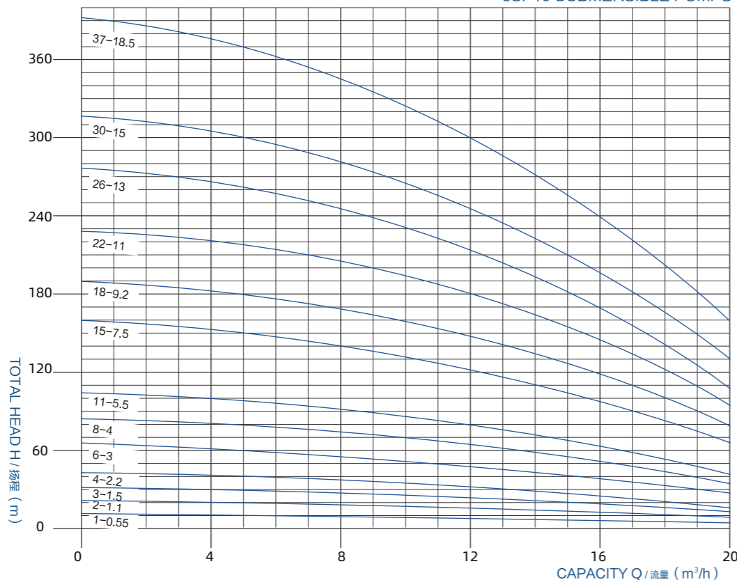
5SP10 SUBMERSIBLE PUMPS
