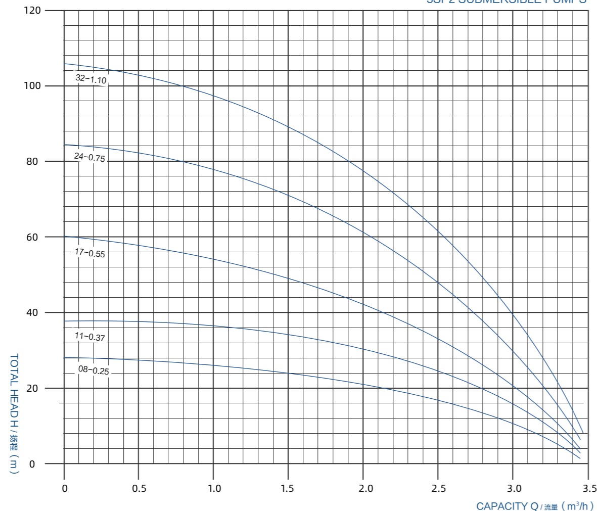
3SP2 SUBMERSIBLE PUMPS
